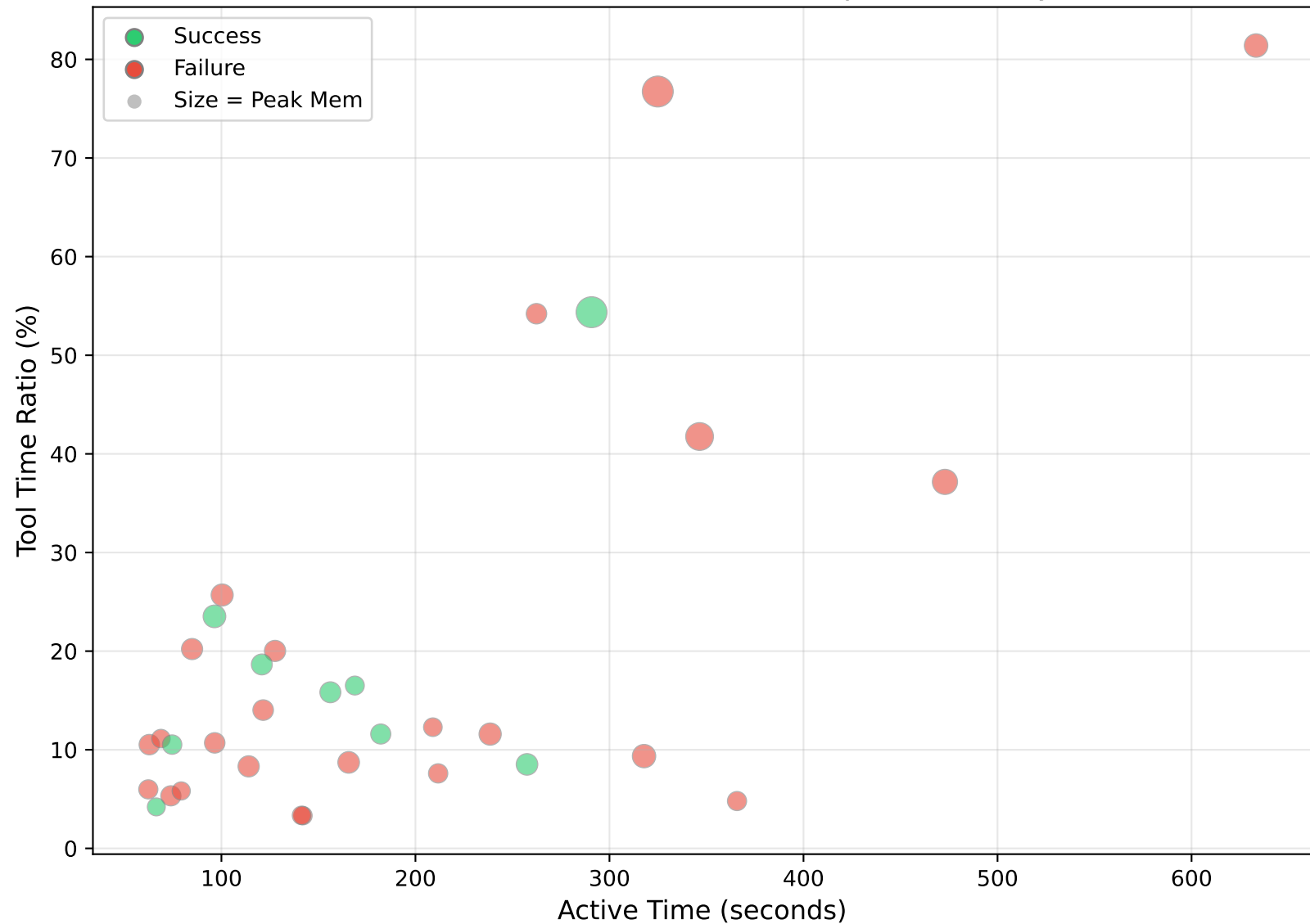
Active Time vs Tool Ratio (size = peak memory)
